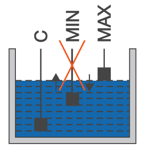
Operation mode with two electrodes
