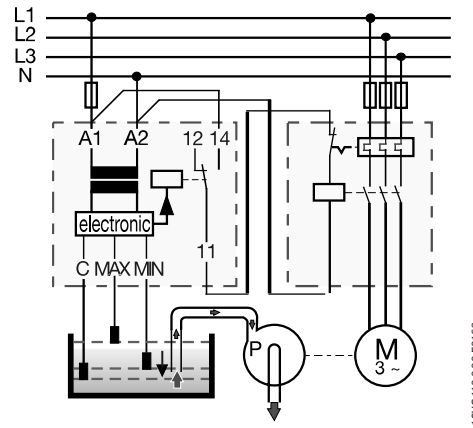
Liquid level control - drain - selected function "↓" (Down)
