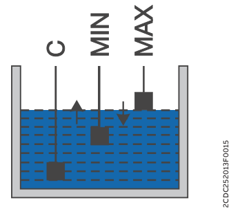
Operation mode with three electrodes
