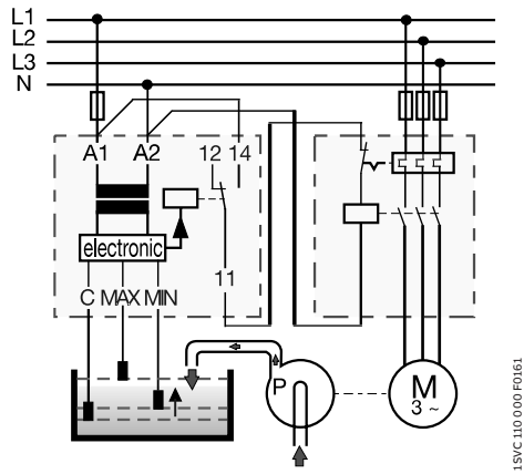
Liquid level control - fill - selected function "↑" (UP)
