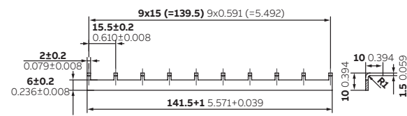
CR-PJ jumper bar
